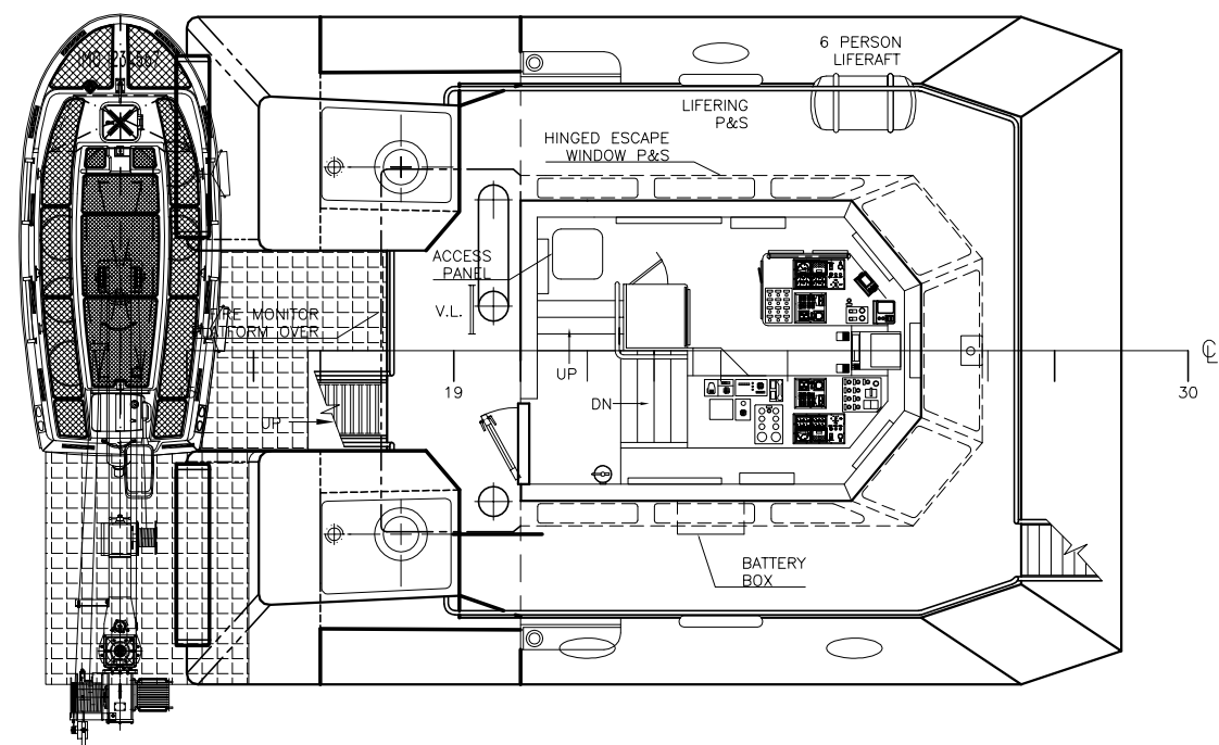
WHEEL HOUSE PLAN
