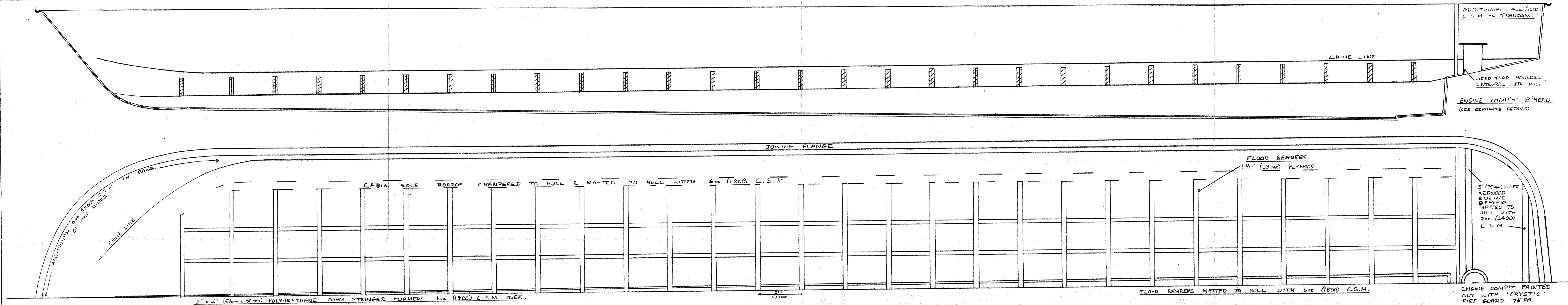
PLAN & ELEVATION OF HULL STIFFENING.
